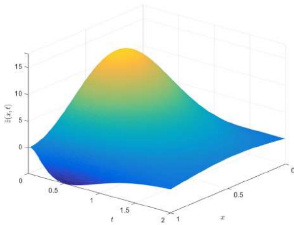
Fig. 5. Boundary control: The estimation/prediction \hat{z}(x, t) .
